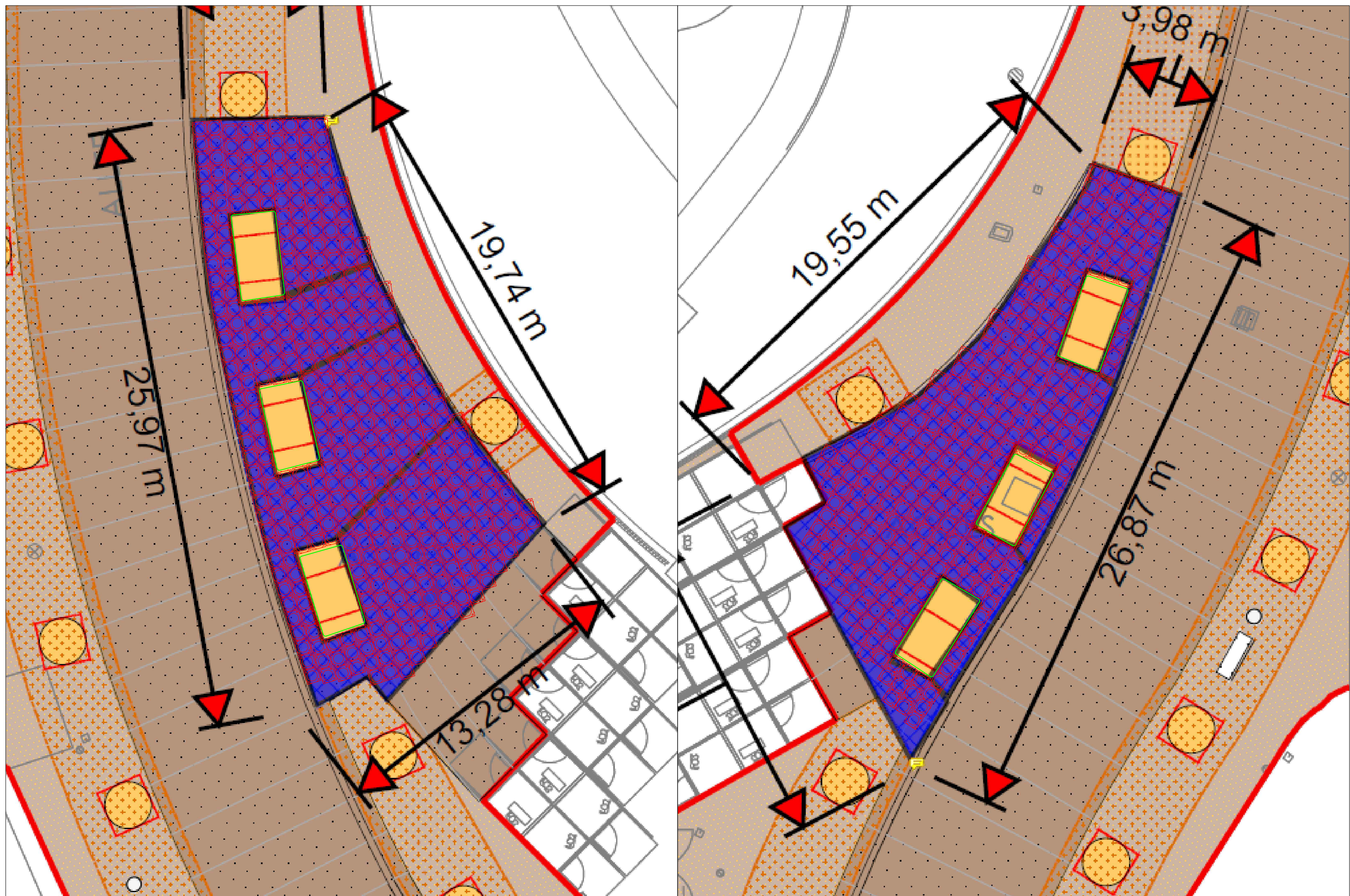
Detail TreeParker system 0.80 m tour eiffel tower option 1
